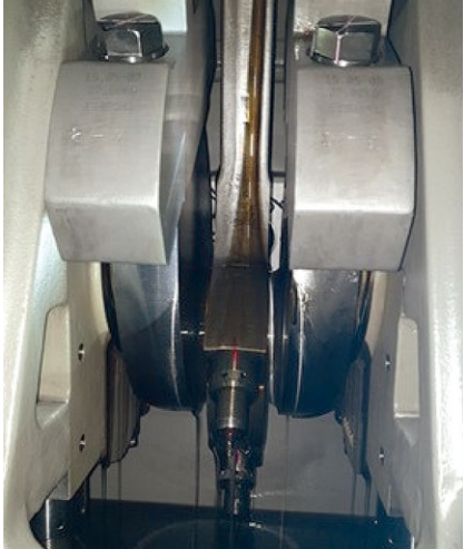
Inspection of Crank Chamber
