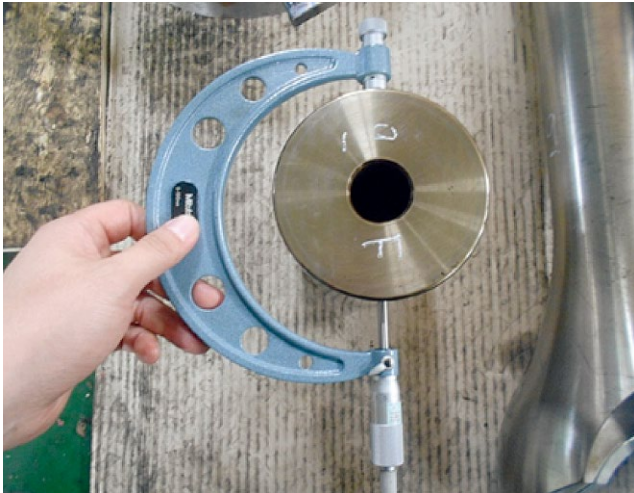
Piston pin measurement
